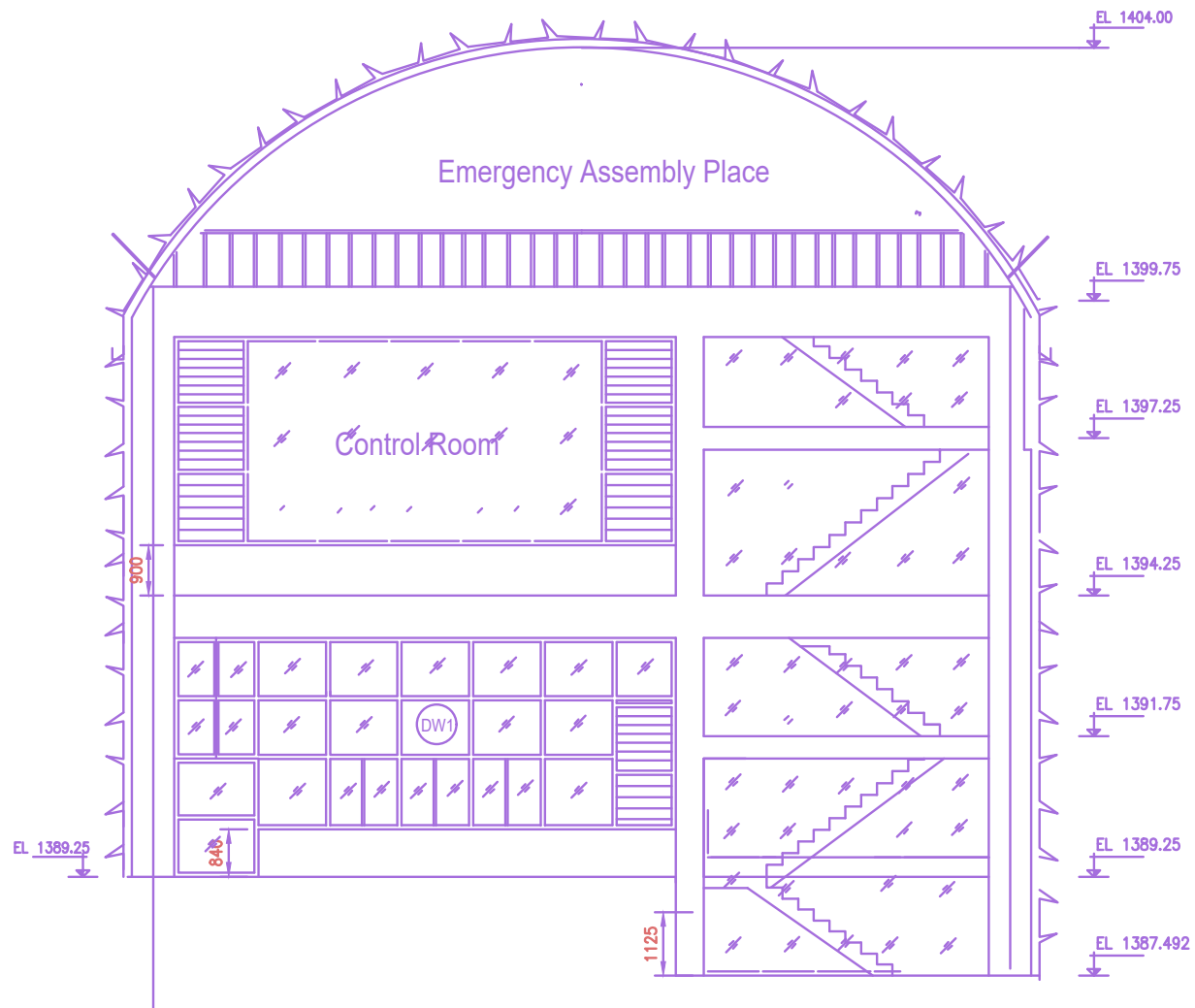
FRONT ELEVATION
